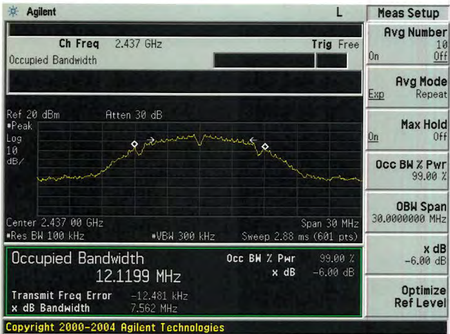
6dB Bandwidth plot on channel 6
