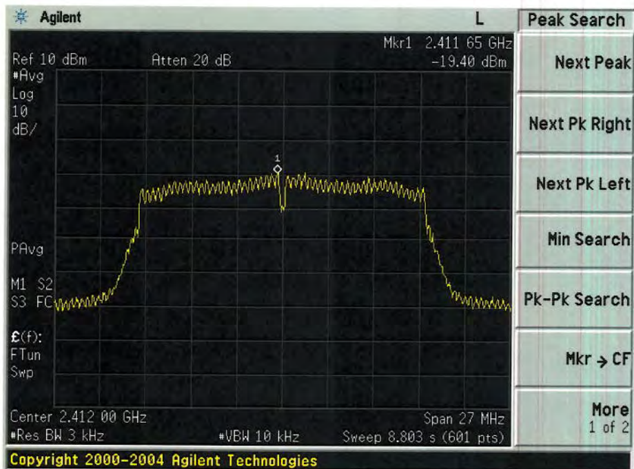
Power spectral density plot on channel 1
