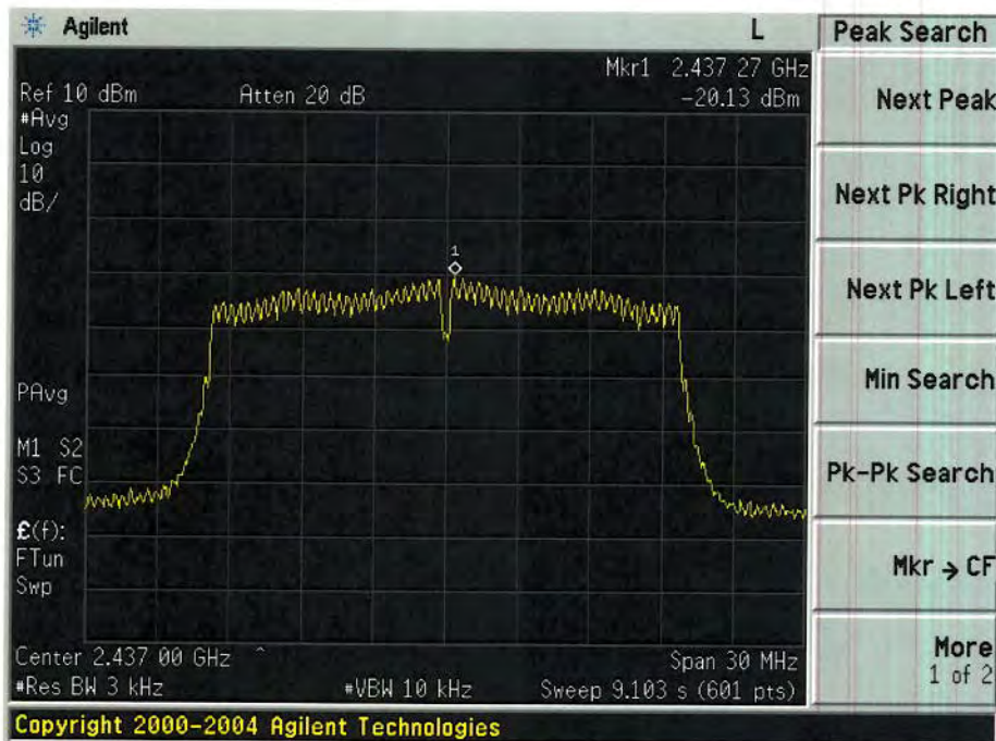
Power spectral density plot on channel 6
